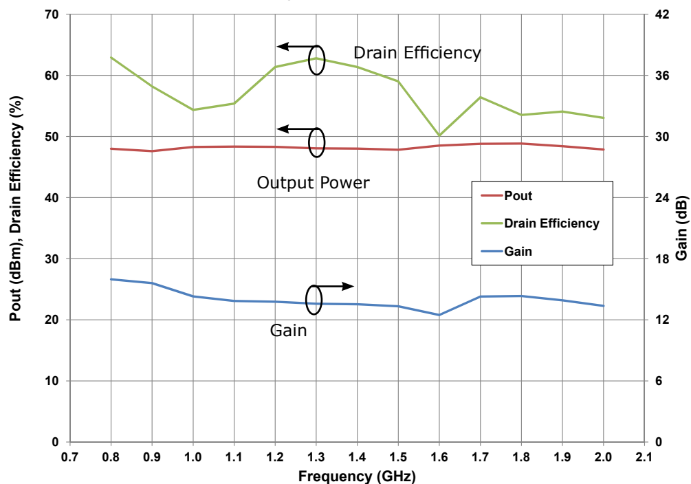
Figure 2. - Gain, Output Power and Drain Efficiency vs Frequency of the CGHV40050 measured in Broadband Amplifier Circuit CGHV40050-TB V_{DD} = 50 \text{ V} , I_{DQ} = 300 \text{ mA} , T_{case} = 25^\circ\text{C}
