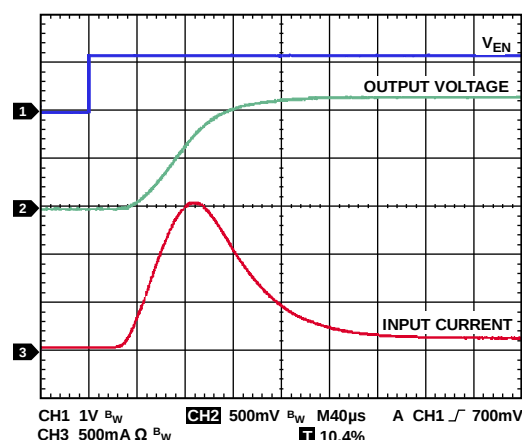
Figure 36. Typical Rise Time and Inrush Current, C_{LOAD} = 100\text{ }\mu\text{F} , V_{IN} = 1.2\text{ V} , I_{LOAD} = 100\text{ mA}
