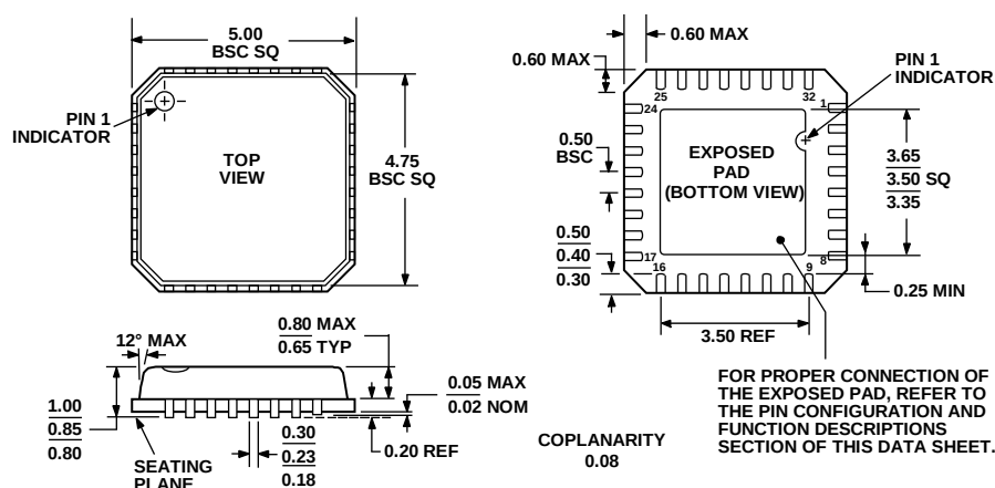
COMPLIANT TO JEDEC STANDARDS MO-220-VHHD-2 Figure 56. 32-Lead Lead Frame Chip Scale Package [LFCSP_VQ] 5 mm × 5 mm Body, Very Thin Quad (CP-32-4) Dimensions shown in millimeters
