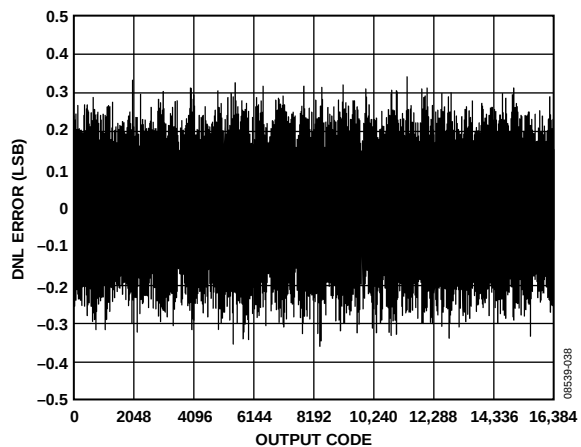
Figure 12. AD9649-80 DNL Error with f_{IN} = 9.7 MHz
