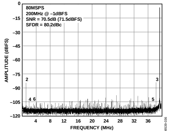
Figure 8. AD9649-80 Single-Tone FFT with f_{IN} = 200 MHz
