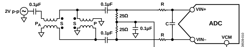
Figure 41. Differential Double Balun Input Configuration
