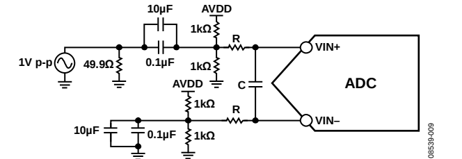
Figure 40. Single-Ended Input Configuration
