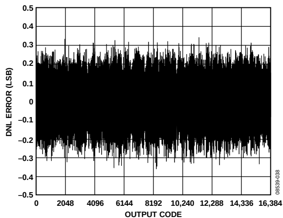
Figure 12. AD9649-80 DNL Error with f_{IN} = 9.7 MHz
