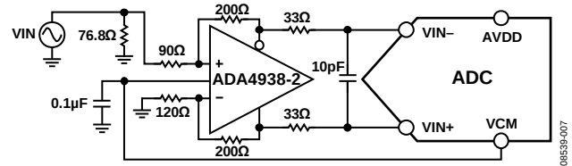
Figure 38. Differential Input Configuration Using the ADA4938-2
