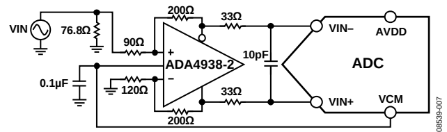
Figure 38. Differential Input Configuration Using the ADA4938-2 For baseband applications below ~10 MHz where SNR is a key parameter, differential transformer coupling is the recommended input configuration. An example is shown in Figure 39. To bias the analog input, the VCM voltage can be connected to the center tap of the secondary winding of the transformer.
