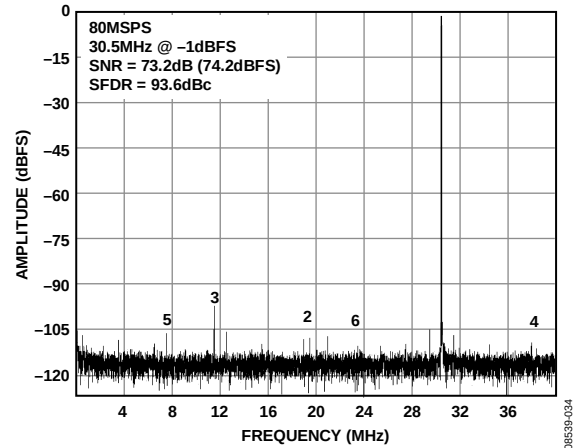
Figure 7. AD9649-80 Single-Tone FFT with f_{IN} = 30.5 MHz
