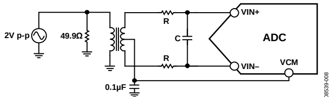
Figure 39. Differential Transformer-Coupled Configuration The signal characteristics must be considered when selecting a transformer. Most RF transformers saturate at frequencies below a few megahertz (MHz). Excessive signal power can also cause core saturation, which leads to distortion. At input frequencies in the second Nyquist zone and above, the noise performance of most amplifiers is not adequate to achieve
