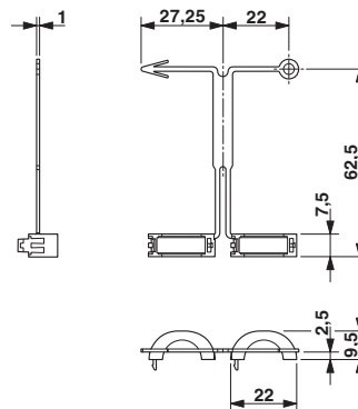
Dimensioned drawing
