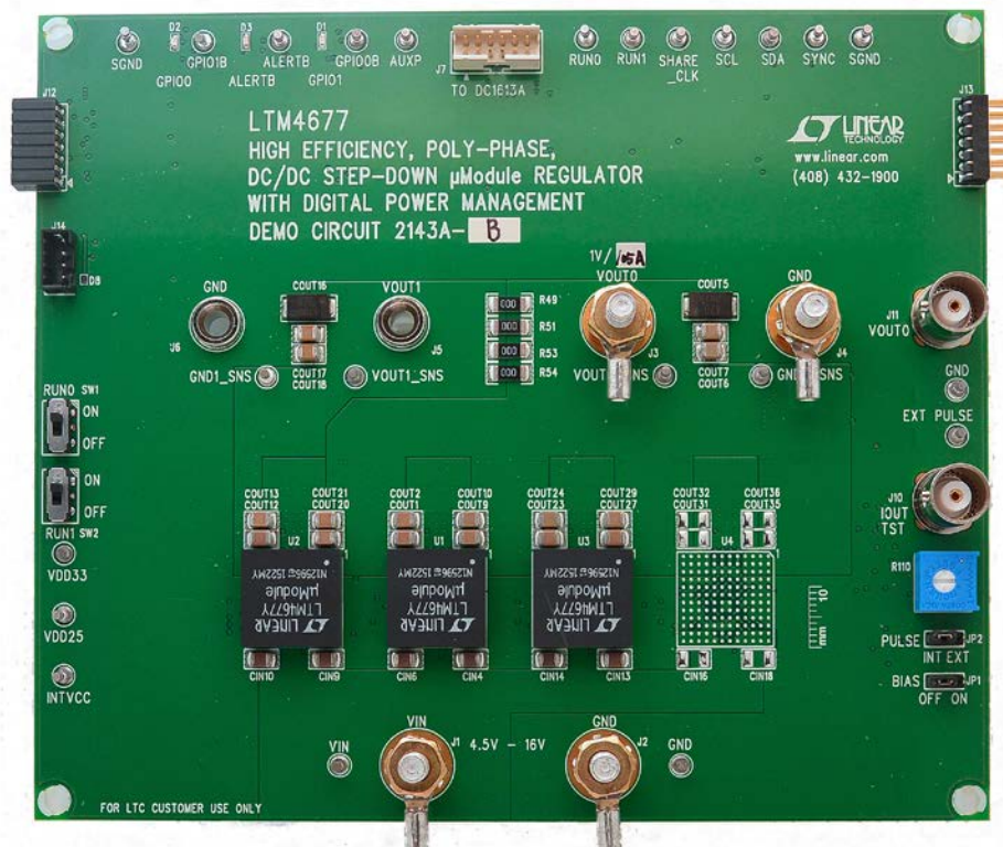
Figure 1. 3 \times LTM4677; 108A DC2143A-B Demo Circuit
