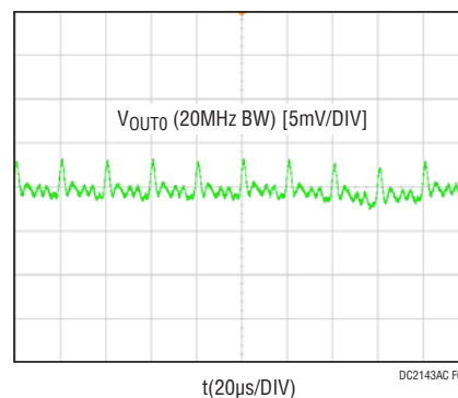
Figure 7. Output Voltage Ripple at V_{IN} = 12V , V_{OUT0} = 1V , I_{OUT0} = 108A , f_{SW} = 500kHz
