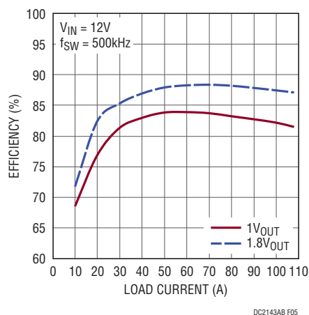
Figure 5. Efficiency vs Load Current for V_{OUT} = 1V and V_{OUT} = 1.8V at V_{IN} = 12V , f_{SW} = 500kHz
