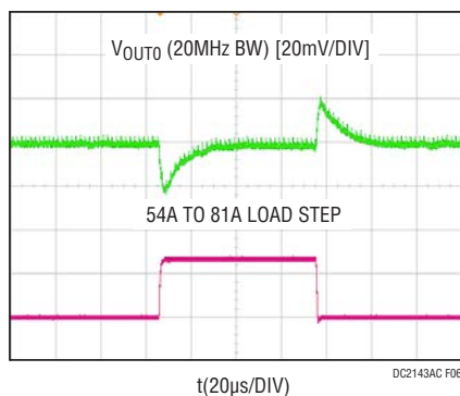
Figure 6. Output Voltage V_{OUT0} vs Load Current at V_{IN} = 12V , V_{OUT0} = 1V , f_{SW} = 500kHz
