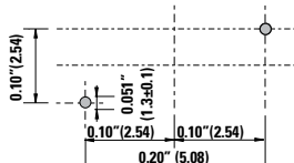
Circuit Board Mounting Detail
