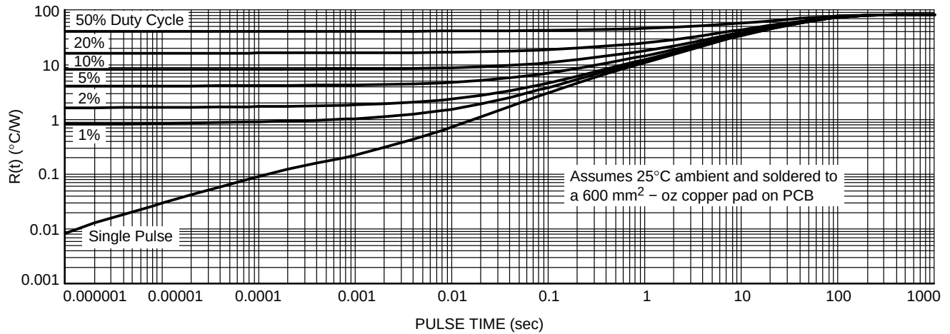
Figure 8. Thermal Characteristics
