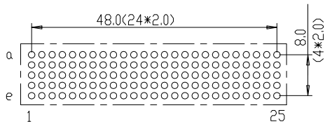
LAY-OUT P.C.B.-HOLE (FRONT SIDE)
