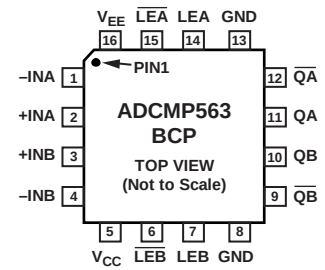
Figure 7. ADCMP563 16-Lead LFCSP Pin Configuration
