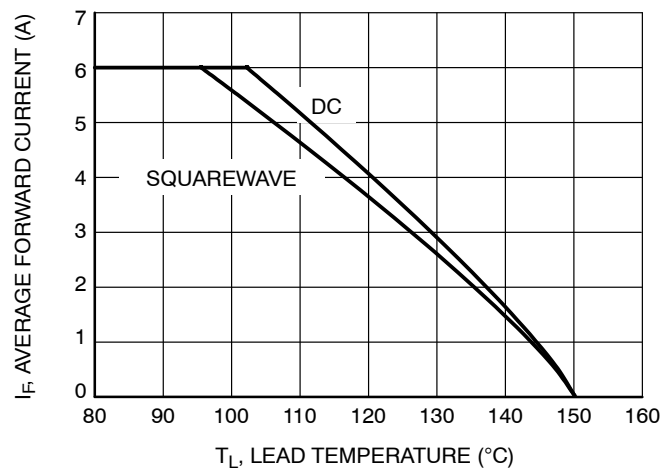
Figure 7. Derating Curve
