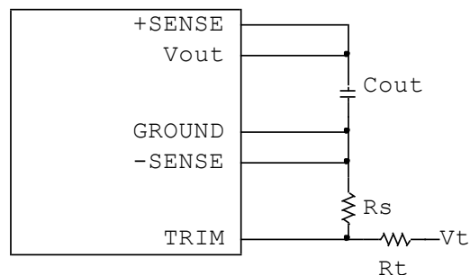
Figure 33: Trim Output Voltage – with Voltage Source
