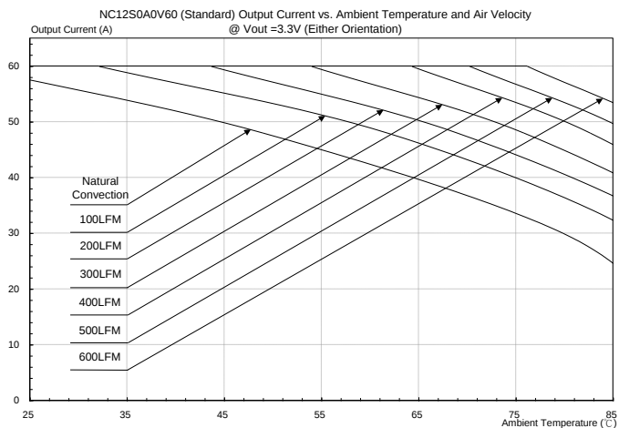
Figure 38: Output current vs. ambient temperature and air hvelocity@ Vout=3.3V(Either Orientation)
