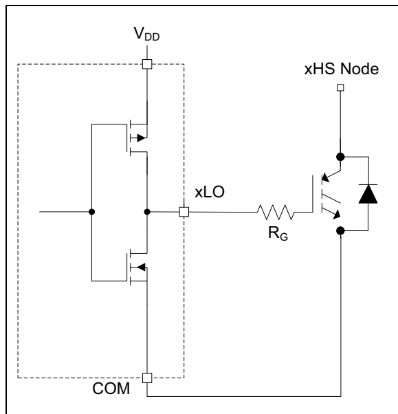
FIGURE 4-5: Low-Side Driver Block Diagram.
