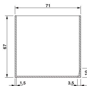
Dimensional drawing
