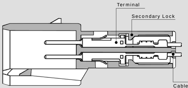
Male Connector
