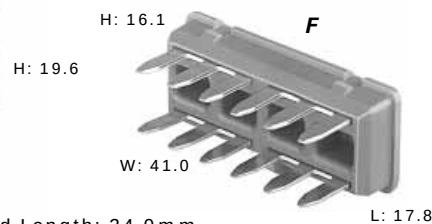
12176478 Cap Assembly 4-3M Mates to Connector 12176473
