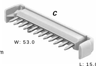
12176469 Cap Assembly 2-6M Mates to Connector 12176460
