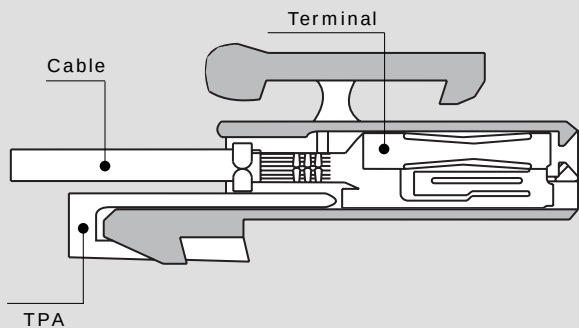
Female Connector
