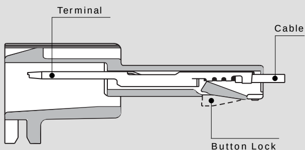
Male Connector
