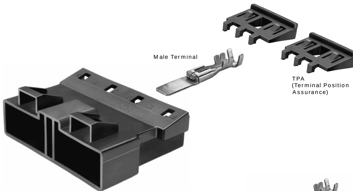
Male Connector
