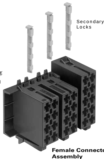
Female Terminal
