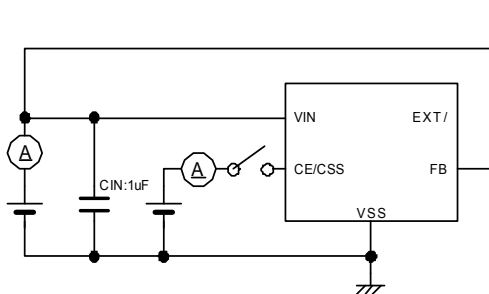
Circuit 1: Supply Current, Stand-by Current, CE Current
