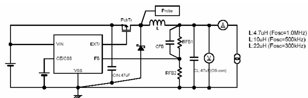
Circuit 3: Oscillation Frequency, PFMDUTY, U.V.L.O., Efficiency
