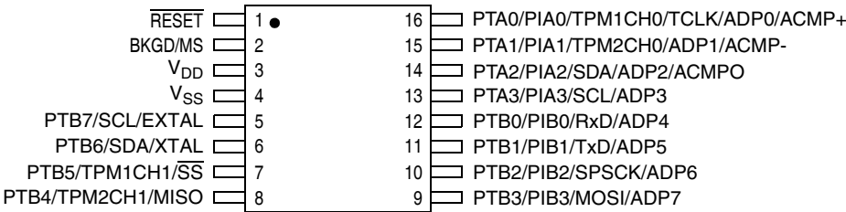
Figure 2-2. 16-Pin TSSOP
