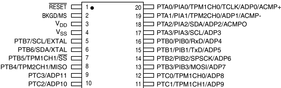
Figure 2-1. 20-Pin TSSOP
