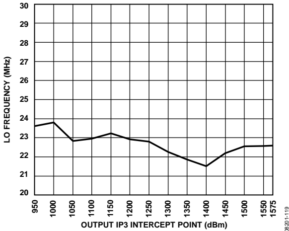
Figure 17. Output IP3 vs. LO Frequency at Nominal Conditions
