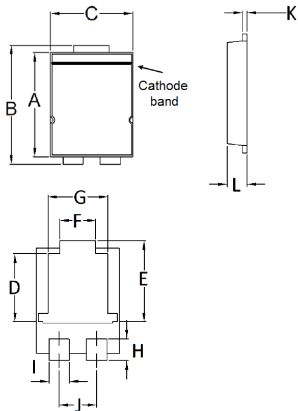
TO-277A (SMPC)
