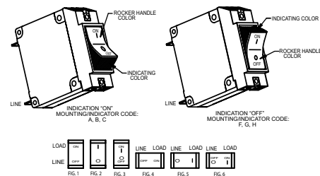
MARKING DETAIL "A"
