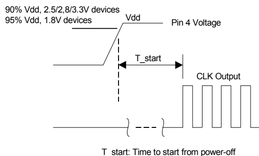
(ST/OE Mode)
