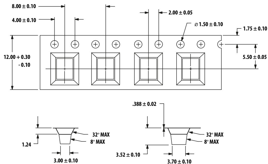
Figure 16: Tape Dimensions
