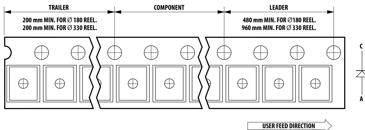
Figure 15: Tape Leader and Trailer Dimensions
