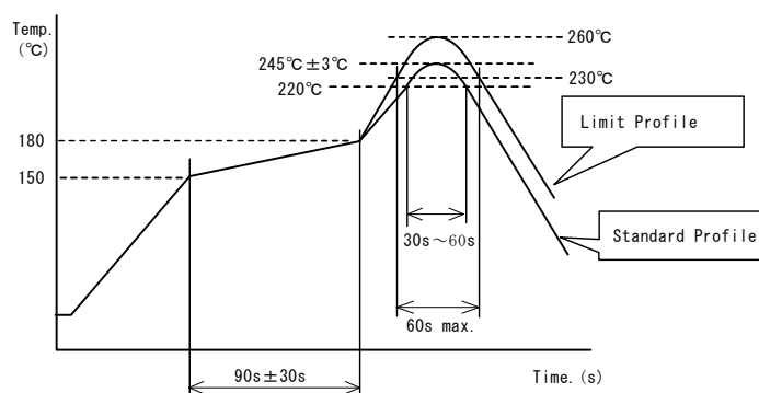
Soldering Profile for Lead Free solder
