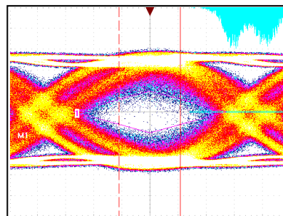
Before ReDriver
