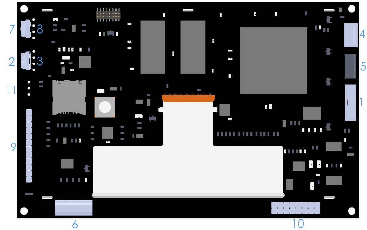
Figure 8: GTT50A Header Locations
