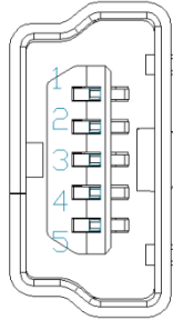
Figure 14: Mass Storage USB Connector
