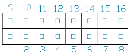
Figure 15: GPO Header
