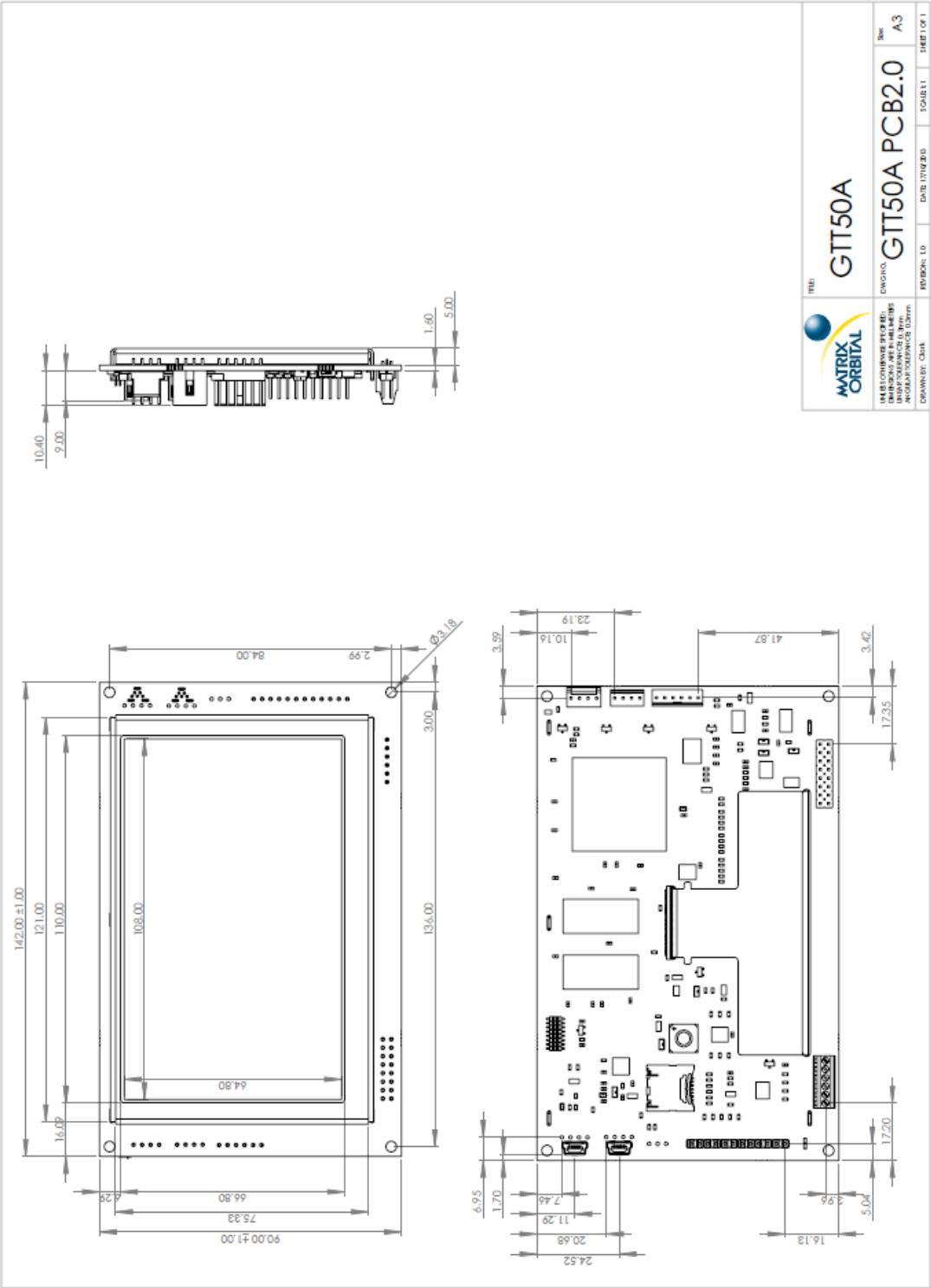
Figure 17: GTT50A Drawing
