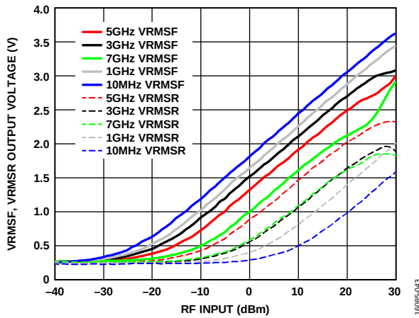
Figure 42. VRMSF, VRMSR Output Voltage vs. RF Input at Various Frequencies When Bridge Driven from RFIN and RFOUT Terminated with 50 \Omega
