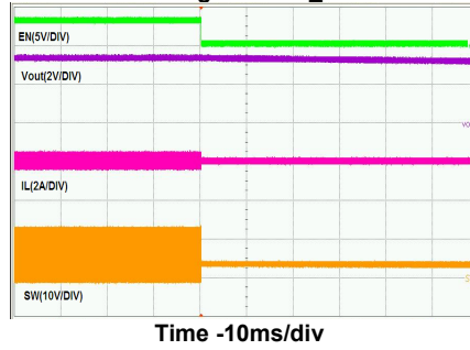
Shutdown Through Enable_no load
