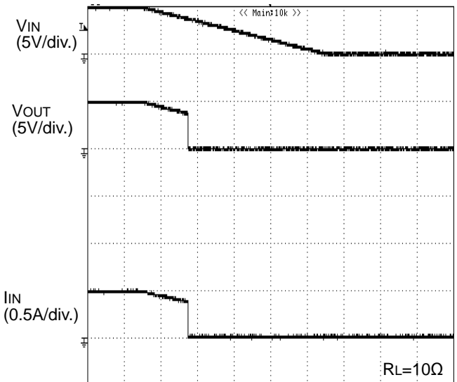
Figure 41. UVLO Response Decreasing VIN
