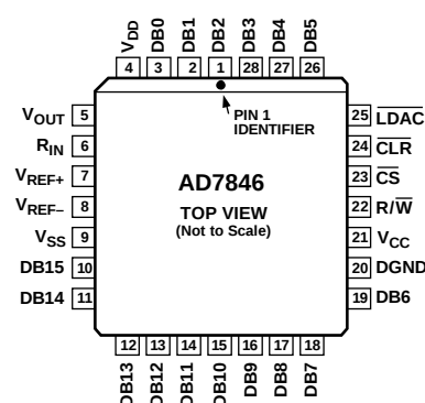
Figure 8. PLCC or LCC Pin Configuration
