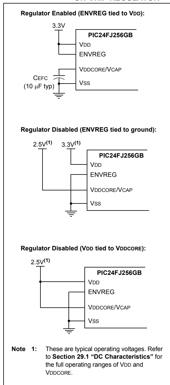
FIGURE 26-1: CONNECTIONS FOR THE ON-CHIP REGULATOR
