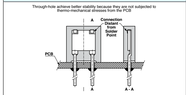
FIGURE 7 – IMPROVED STABILITY WITH THROUGH-HOLE
