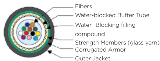
OSP Armored Single Loose Tube Cable
