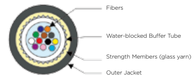
OSP Dielectric Single Loose Tube Cable
