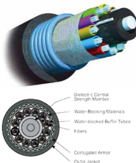
OSP Armored Stranded Loose Tube Cable
