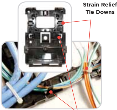
Fiber Loop Management
