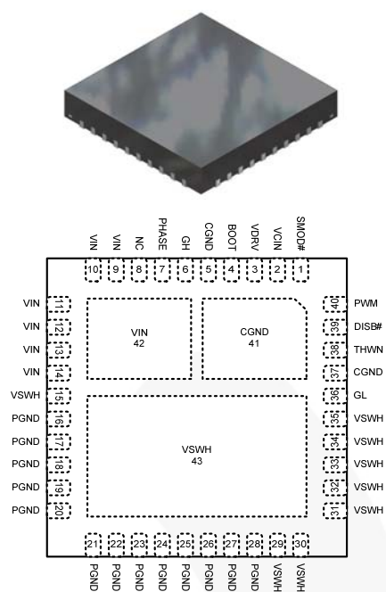
Figure 4. Top View
