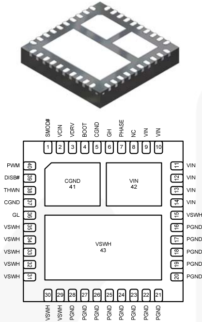
Figure 3. Bottom View
