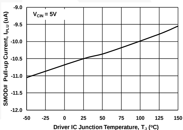
Figure 21. SMOD# Pull-Up Current vs. Temperature
