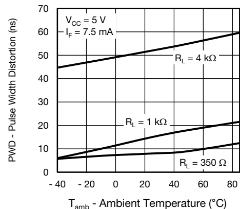
Fig. 14 - Pulse Width Distortion vs. Ambient Temperature
