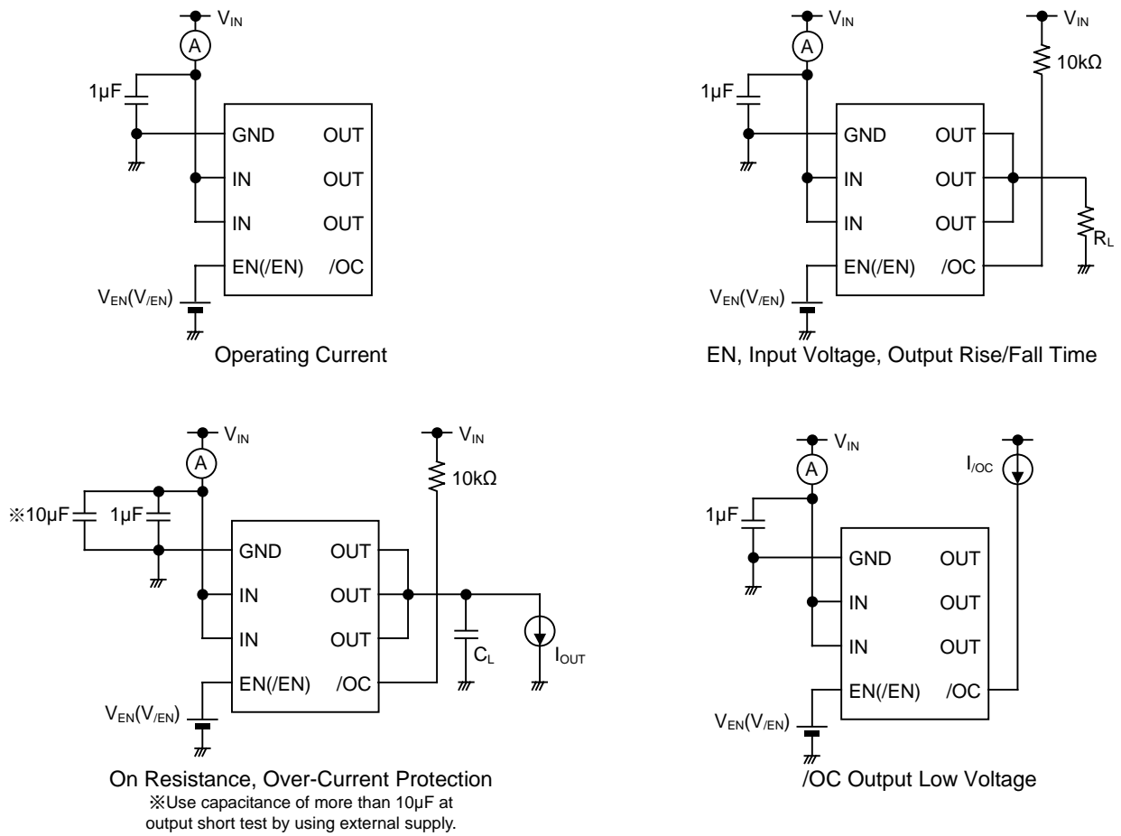
Figure 4. Measurement Circuit
