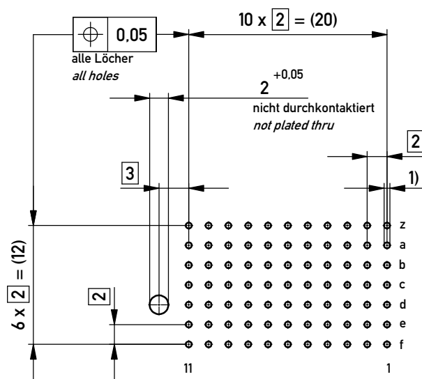
board hole pattern (component mounting side)
