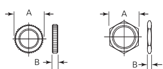
Knurled Nut
