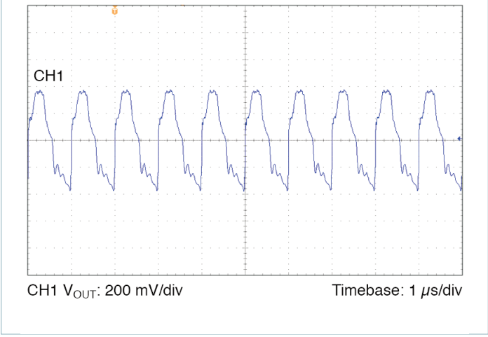
Figure 16 — Output voltage ripple, V_{IN} = 270\text{ V} , V_{OUT} = 24.0\text{ V} , C_{OUT\_EXT} = 220\text{ }\mu\text{F} , R_{LOAD} = 1.152\text{ }\Omega
