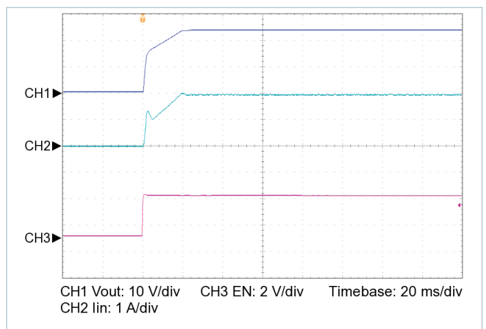
Figure 14 — Startup from EN, V_{IN} = 270\text{ V} , C_{OUT\_EXT} = 2200\text{ }\mu\text{F} , R_{LOAD} = 1.152\text{ }\Omega
