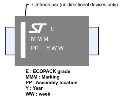
Figure 19. Marking layout
