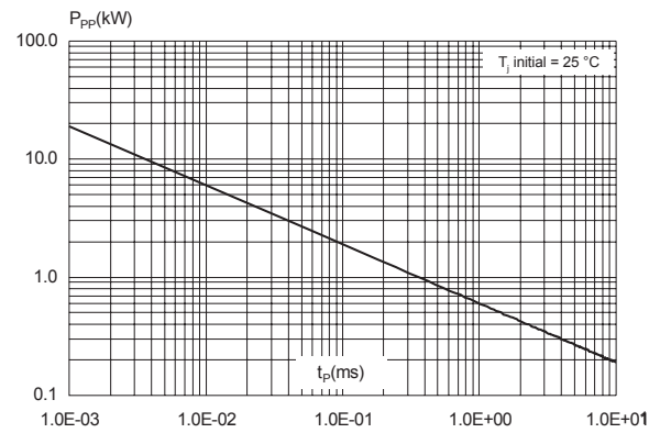
Figure 5. Maximum peak pulse power versus exponential pulse duration
