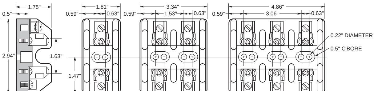
Figure 2. 31 to 60A
