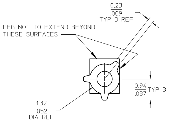
PEG DETAIL SCALE 10 : 1
