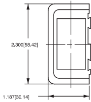
VME MOUNTING PANEL END
