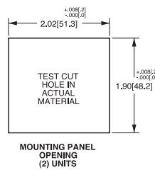
VMS MOUNTING HOLE
