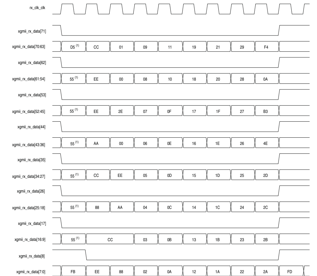
Figure 9–7. SDR XGMII RX Interface Data Bus
