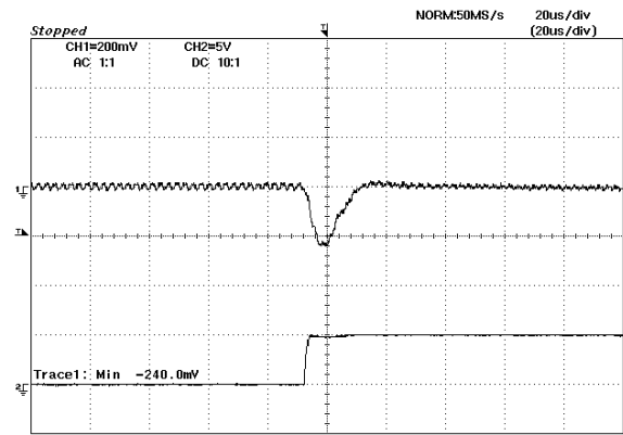
Figure 14: Typical transient response to step load change at 2.5\text{A}/\mu\text{s} from 50% to 100% of I_o , max at 12Vin, 5.0V out ( C_{out} = 1\mu\text{F} ceramic, 10\mu\text{F} tantalum) I_o:2\text{A}/\text{DIV}
