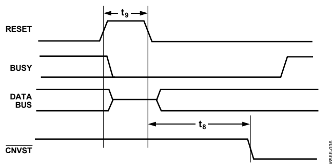
Figure 36. RESET Timing
