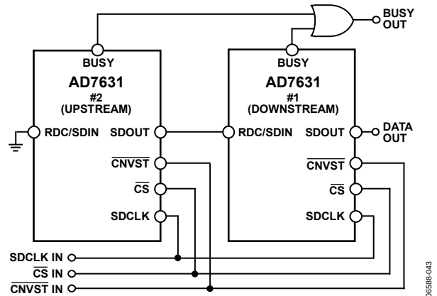
Figure 43. Two AD7631 Devices in a Daisy-Chain Configuration
